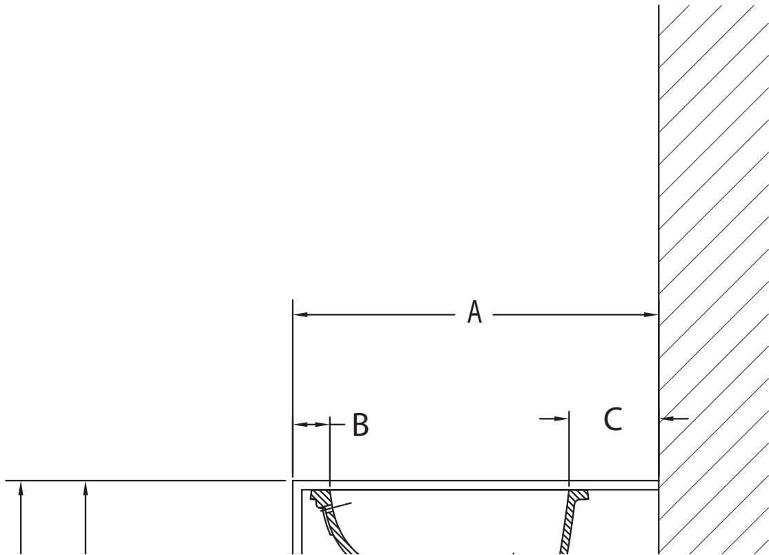
Figure I-2: DuPont™ Corian® 830 installation without Skirt
