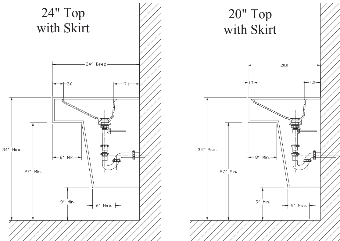
Figure K-4: DuPont™ Corian® 8252 installation with Skirt
