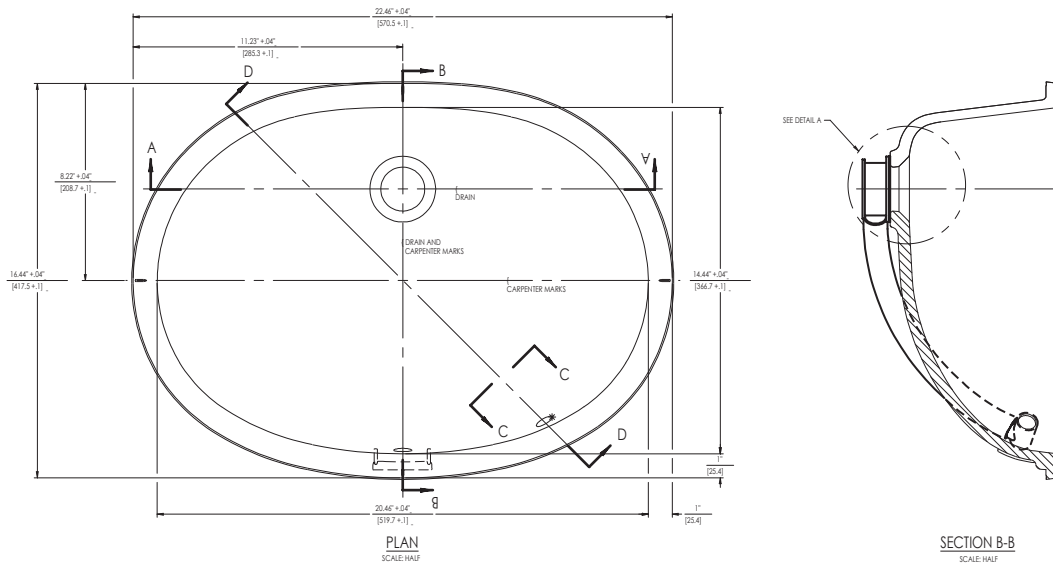
Figure F-2: DuPont™ Corian® 815 with Offset Overflow
