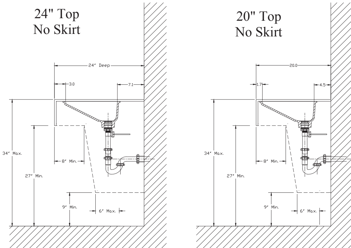
Figure K-3: DuPont™ Corian® 8252 installation without Skirt
