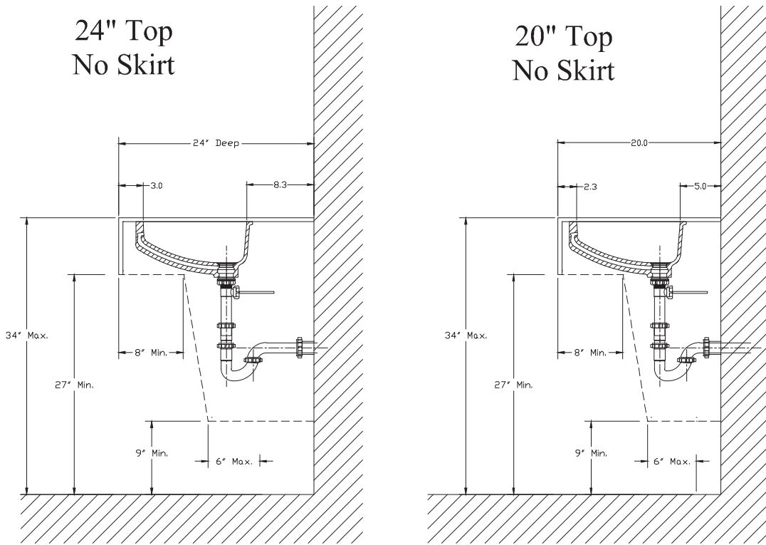
Figure L-3: DuPont™ Corian® 8254 installation without Skirt
