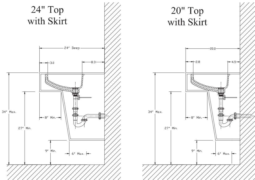
Figure L-4: DuPont™ Corian® 8254 installation with Skirt
