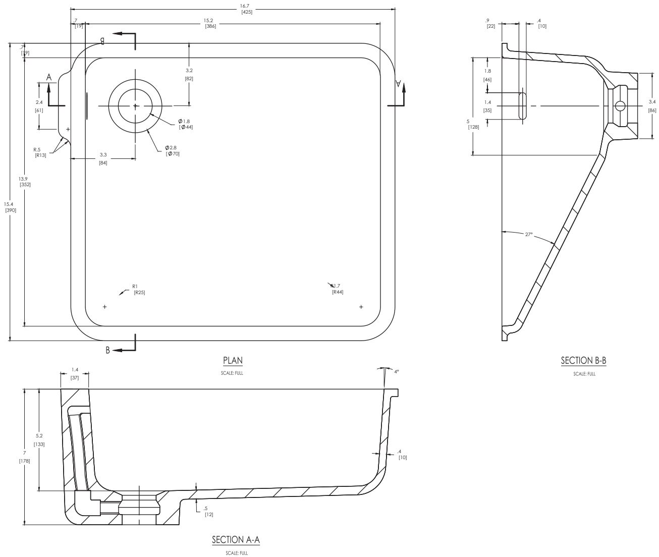
Figure K-1: DuPont™ Corian® 8252 with Overflow
