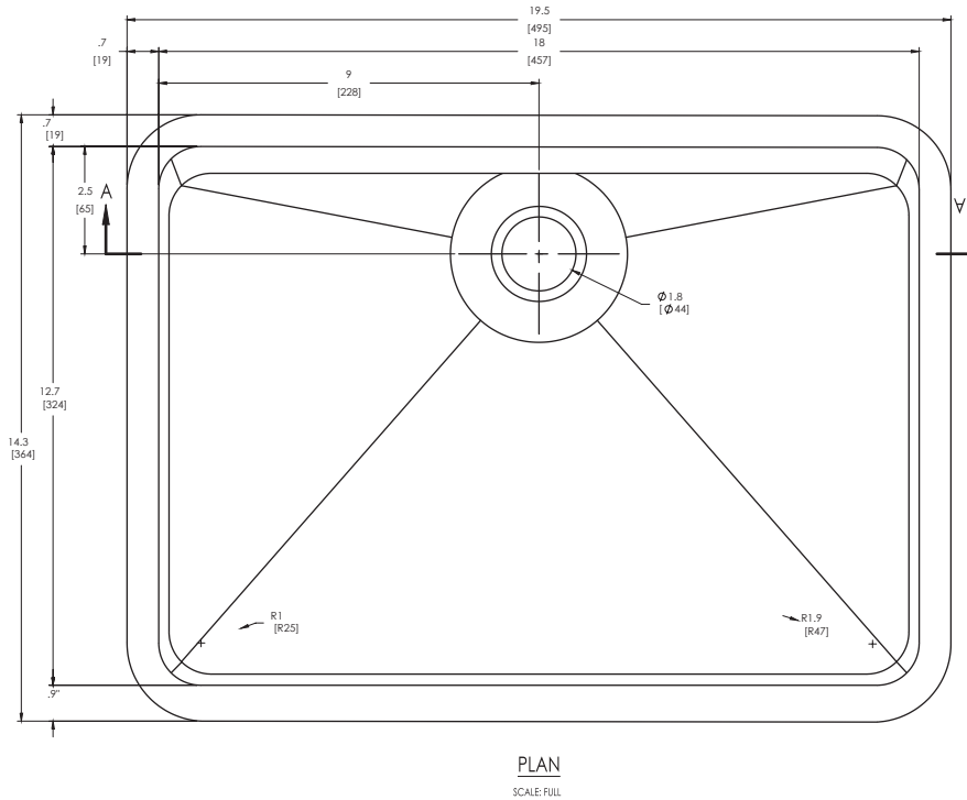
Figure L-1: DuPont™ Corian® 8254 with Integrated Front Overflow
