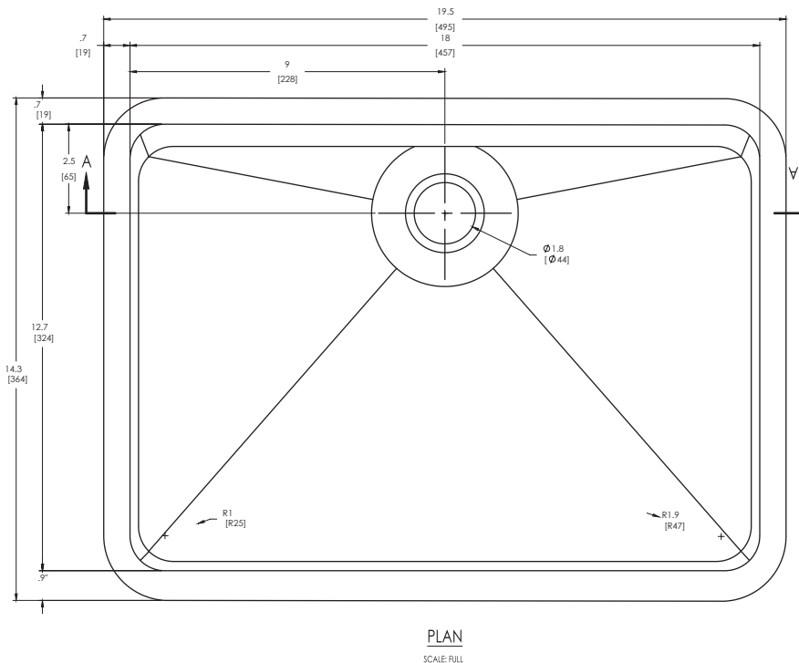
Figure L-2: DuPont™ Corian® 8254 with No Overflow
