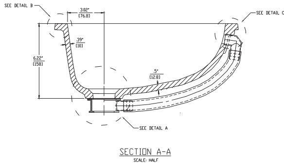
Figure D-1: DuPont™ Corian® 810 with Front Overflow
